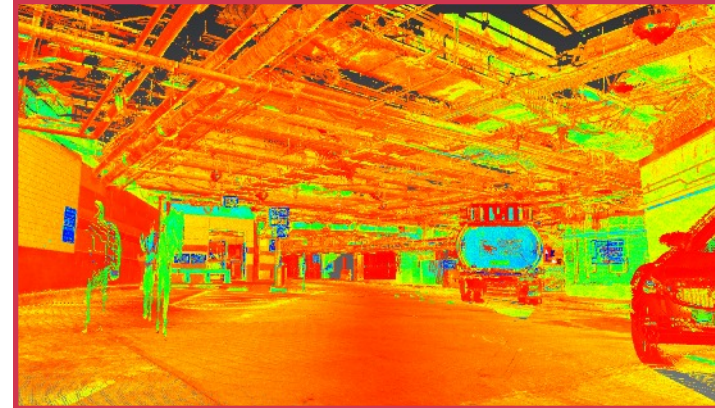
High Definition Survey Point Cloud of Cleveland IX Center
